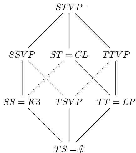
Figure 2: Mixed Consequence for Vague Predicates
