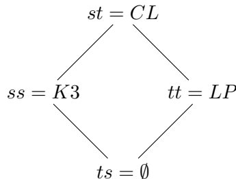
Figure 1: Mixed consequence based on s and t
