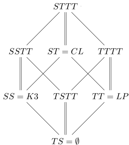
Figure 3: Mixed Consequence for Transparent Truth
